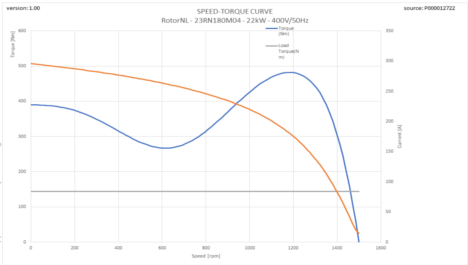
Tn graph
