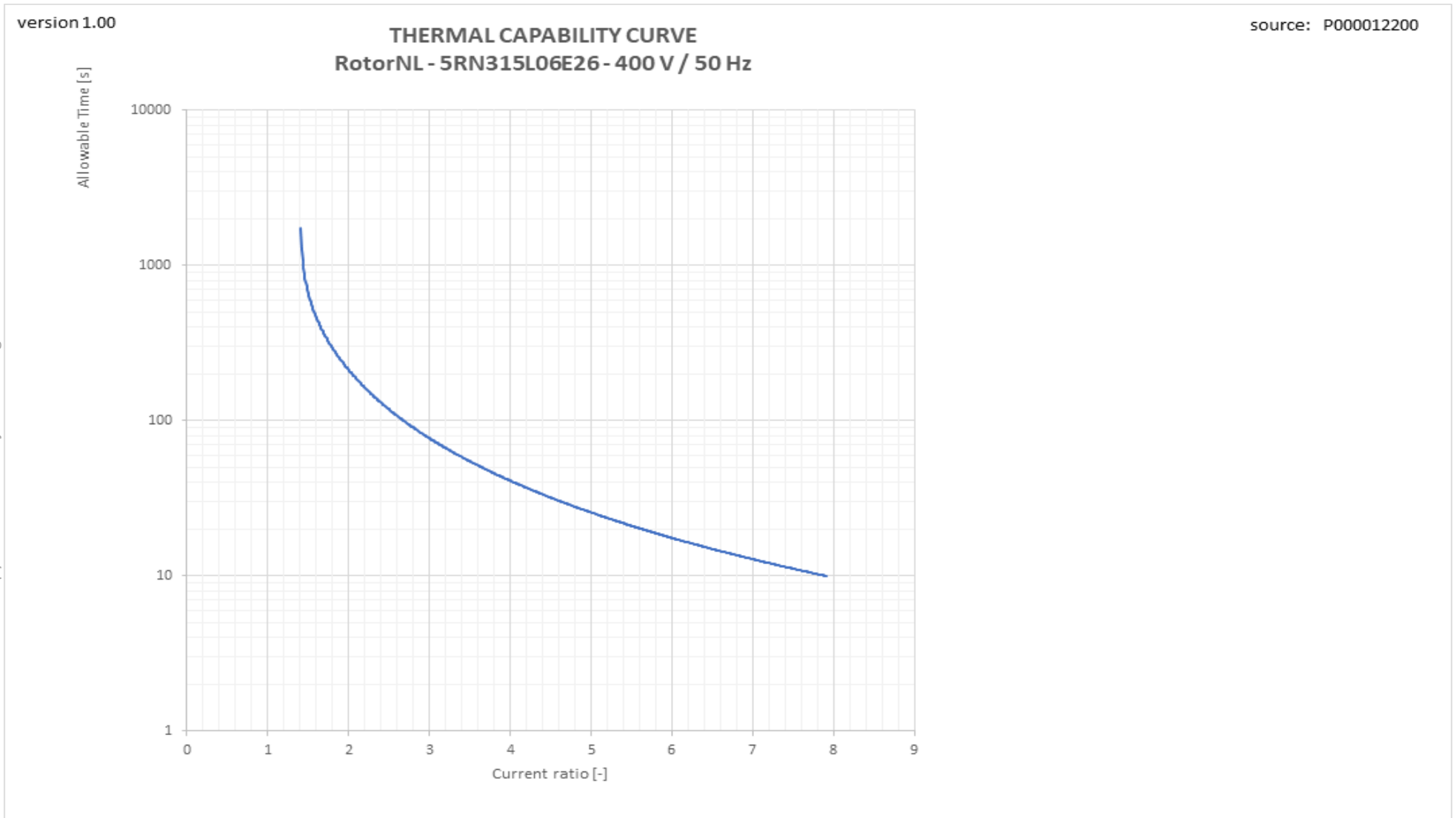
Therm_VSD graph
