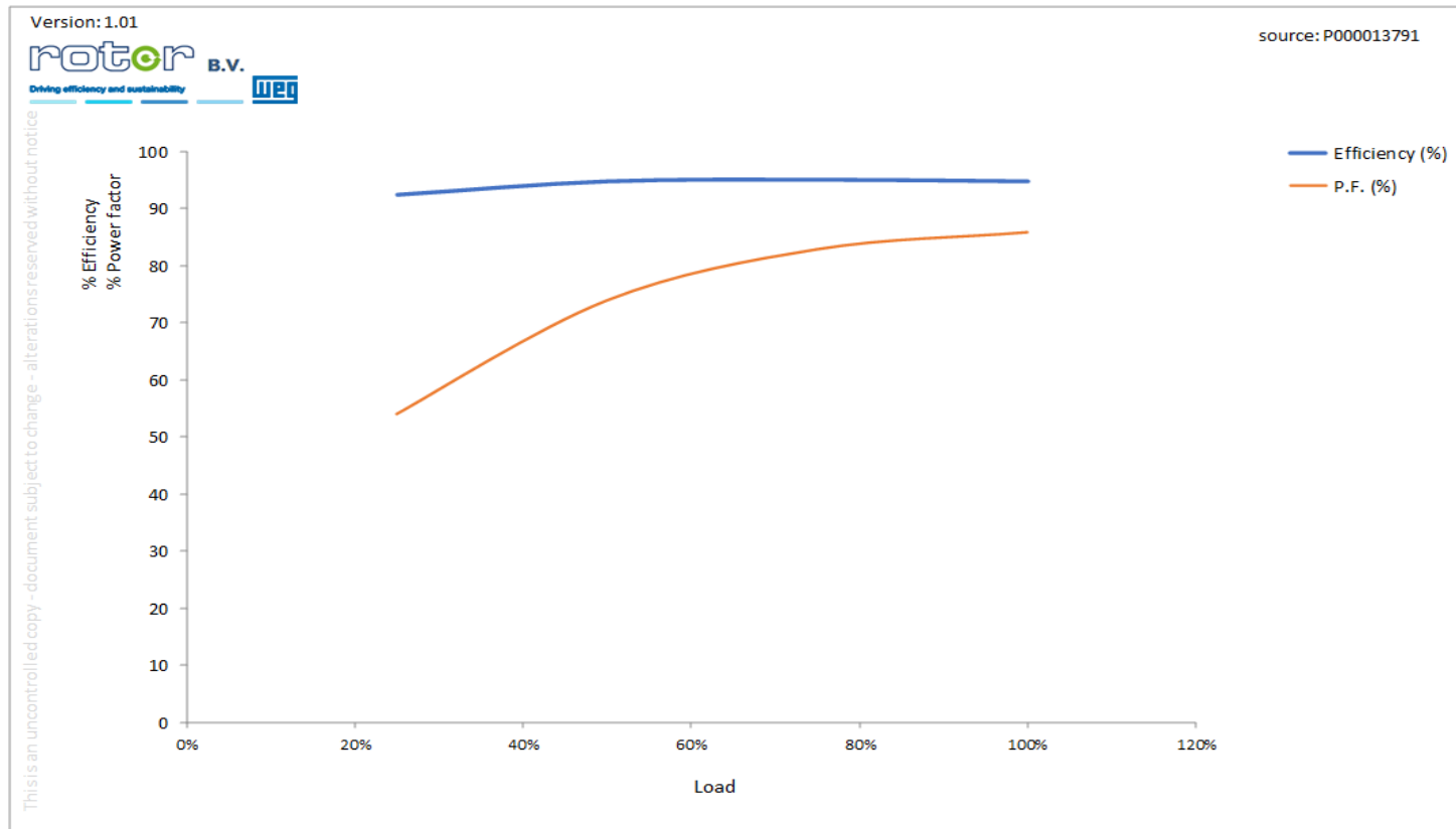
Eff_ & PF graph
