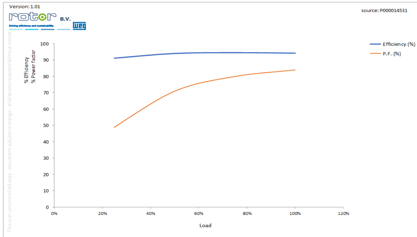
Eff_&_PF graph
