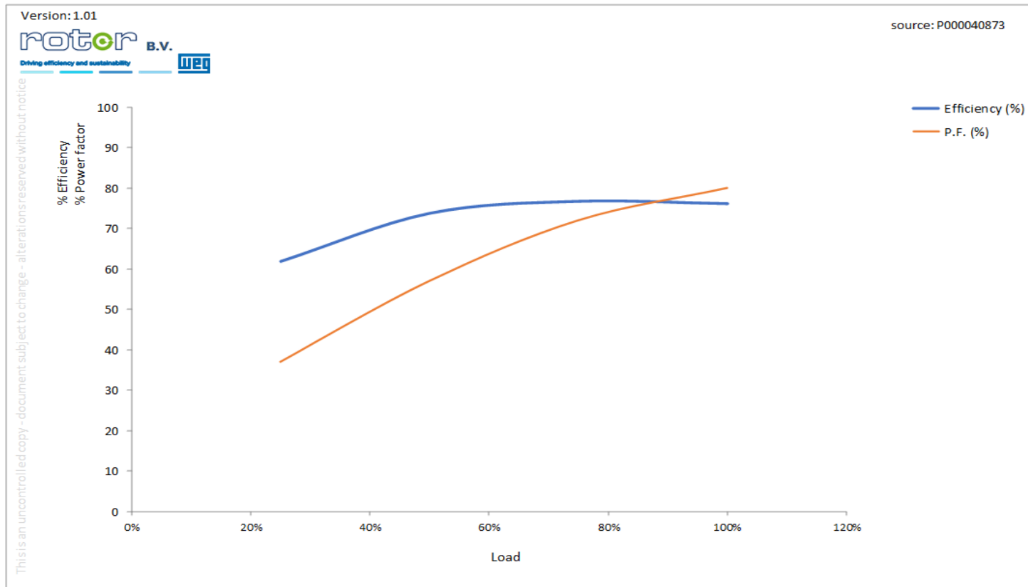
Eff_&_PF graph
