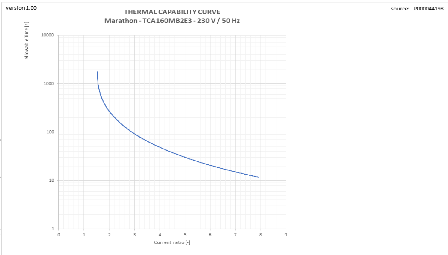
Therm_VSD graph
