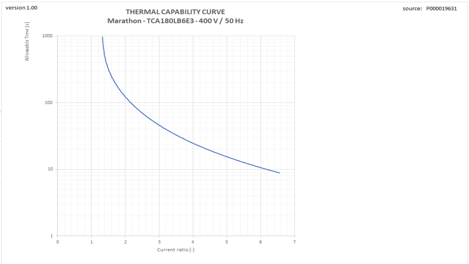
Therm_VSD graph
