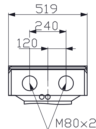
Terminal box - Front view (Simplified detail)
