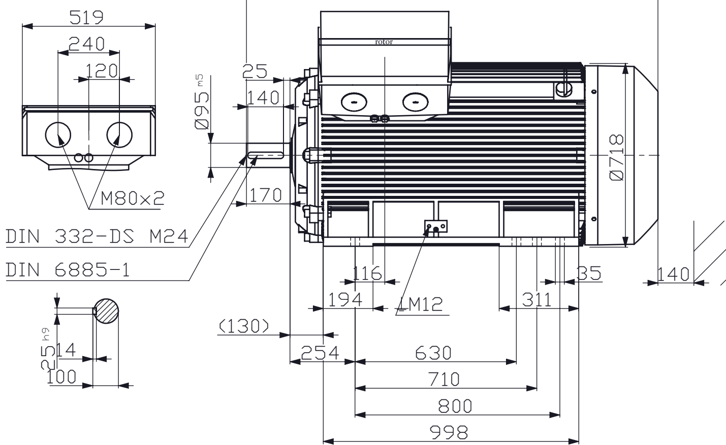
Terminal box - Front view (Simplified detail)
